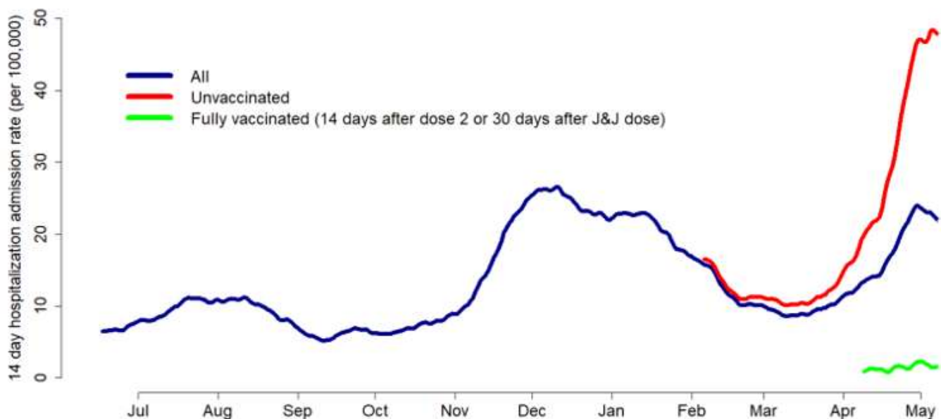
Hospitalization rate by vaccine status in those 45 to 64
